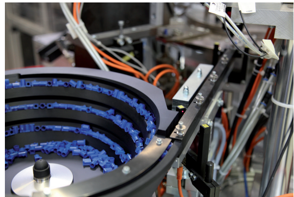
Full automatic SMBA® (FAKRA) feeding
